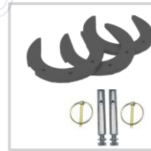
(1) 25# Horseshoe Wt. #HPA0032-1P Mounting Pin Kit #HP0023 Best when used with 11:1 XHD Gear Models
